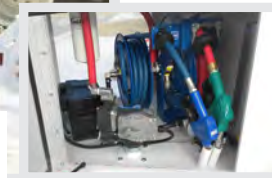
Inside 500FB-DEF Box with DC Pump
